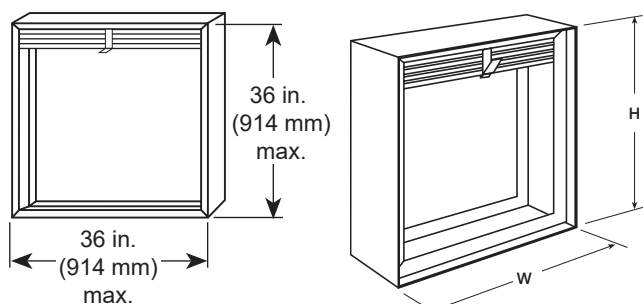
Type A Single Section
