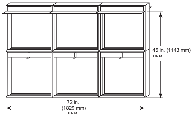
Multi Section Limitations - Type B/B2
