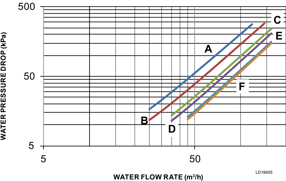
YLAA EVAPORATOR PRESSURE DROP CURVE
