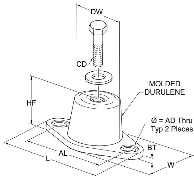
RD3 ISOLATORS
