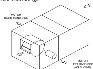
Motor Handling
