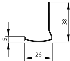
Front border – longitudinal section (L) 26 mm
