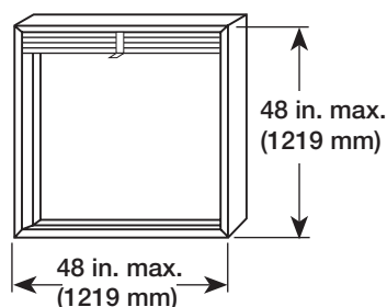
Type A Single Section
