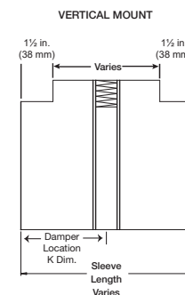
Type B2 side view
